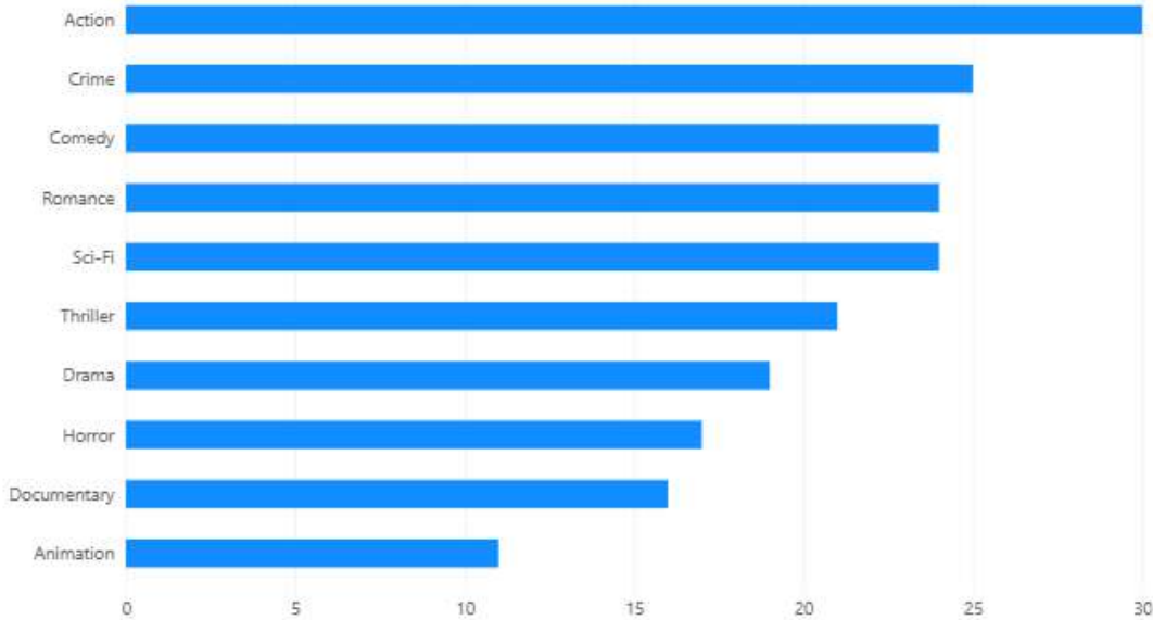
Total Customers by Genre
