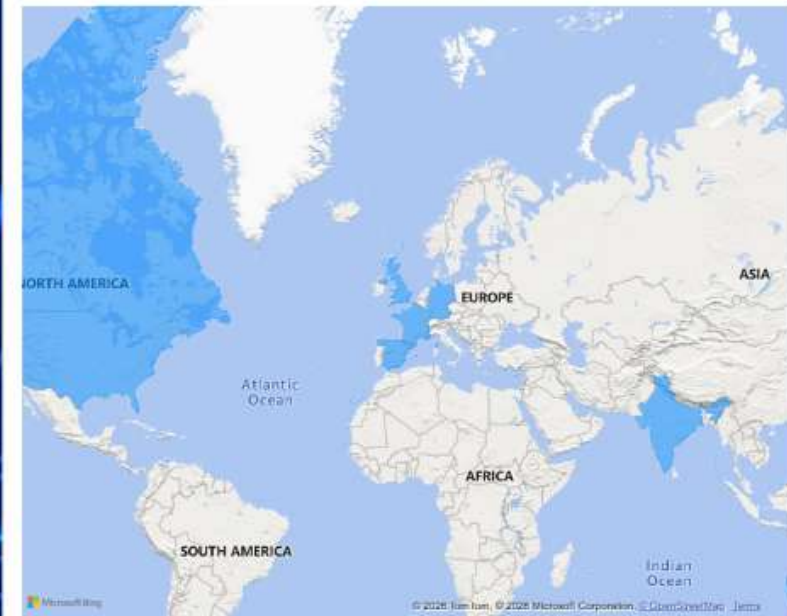
Total Customers by Country
