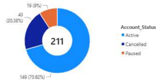
Total Customers by Account_Status
